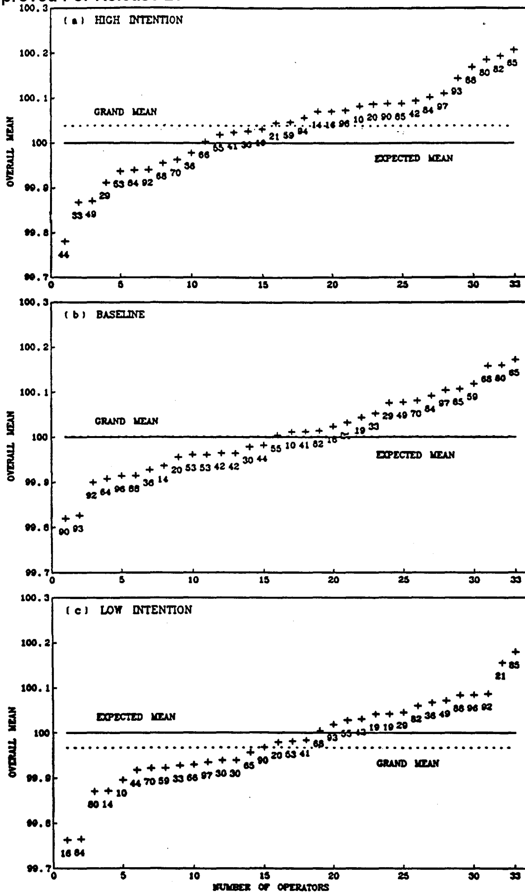
FIGURE 1: 200-SAMPLE REG, ASCENDING OPERATOR MEANS
