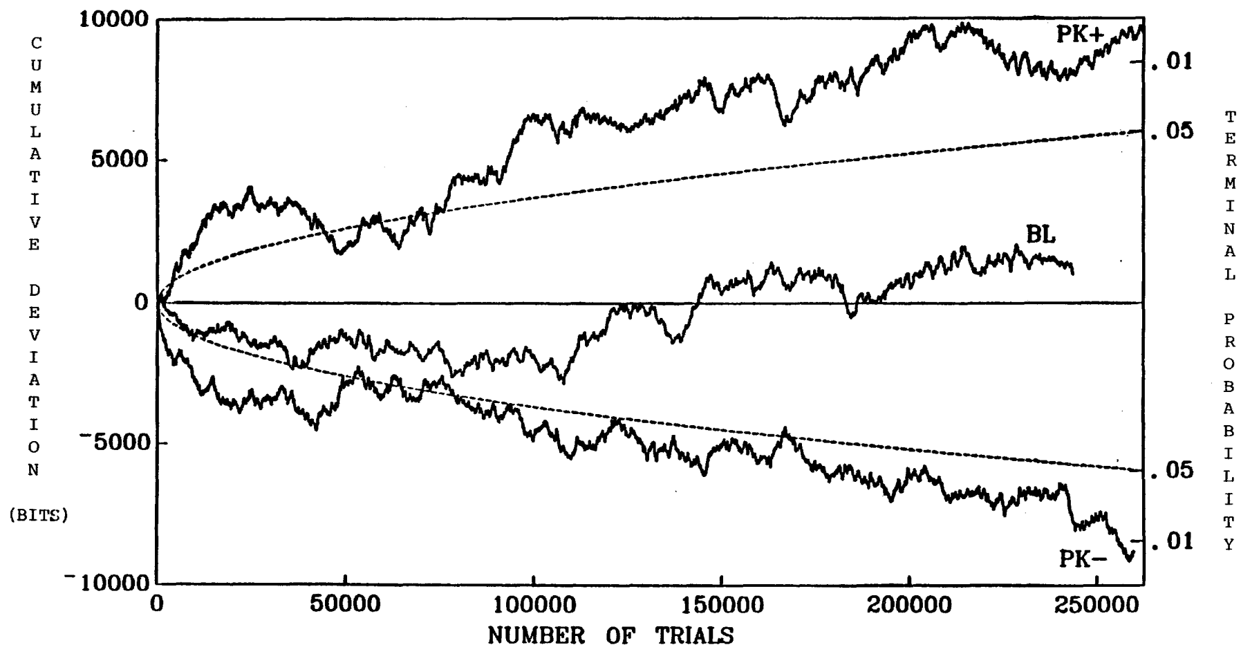
FIGURE 2: CUMULATIVE REG RESULTS, ALL OPERATORS (33), ALL SERIES (87)
